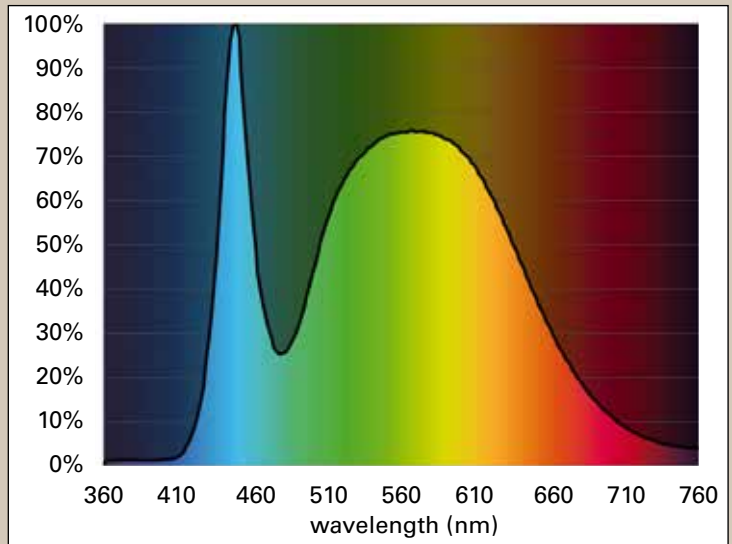
Figure 11. Spectrum of cool (5000K) LED light.
