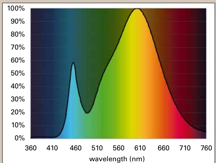
Figure 12. Spectrum of warm (2700K) LED light.
