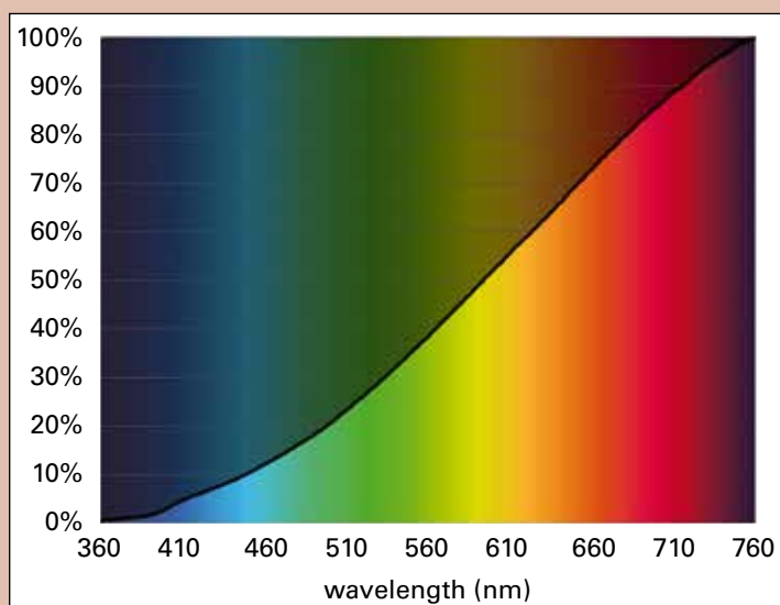
Figure 8. Spectrum of incandescent light.
