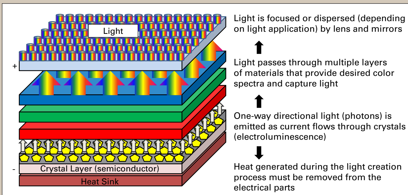
Figure 17. How LED light is created.
